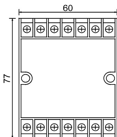
Top View Dimensions in mm
